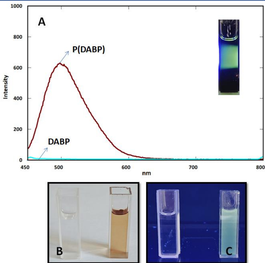
Figure 3. A) Fluorescence spectra B) Image under daylight C) Image under UV light of DABP and P(DABP) (solvent: DMSO)
