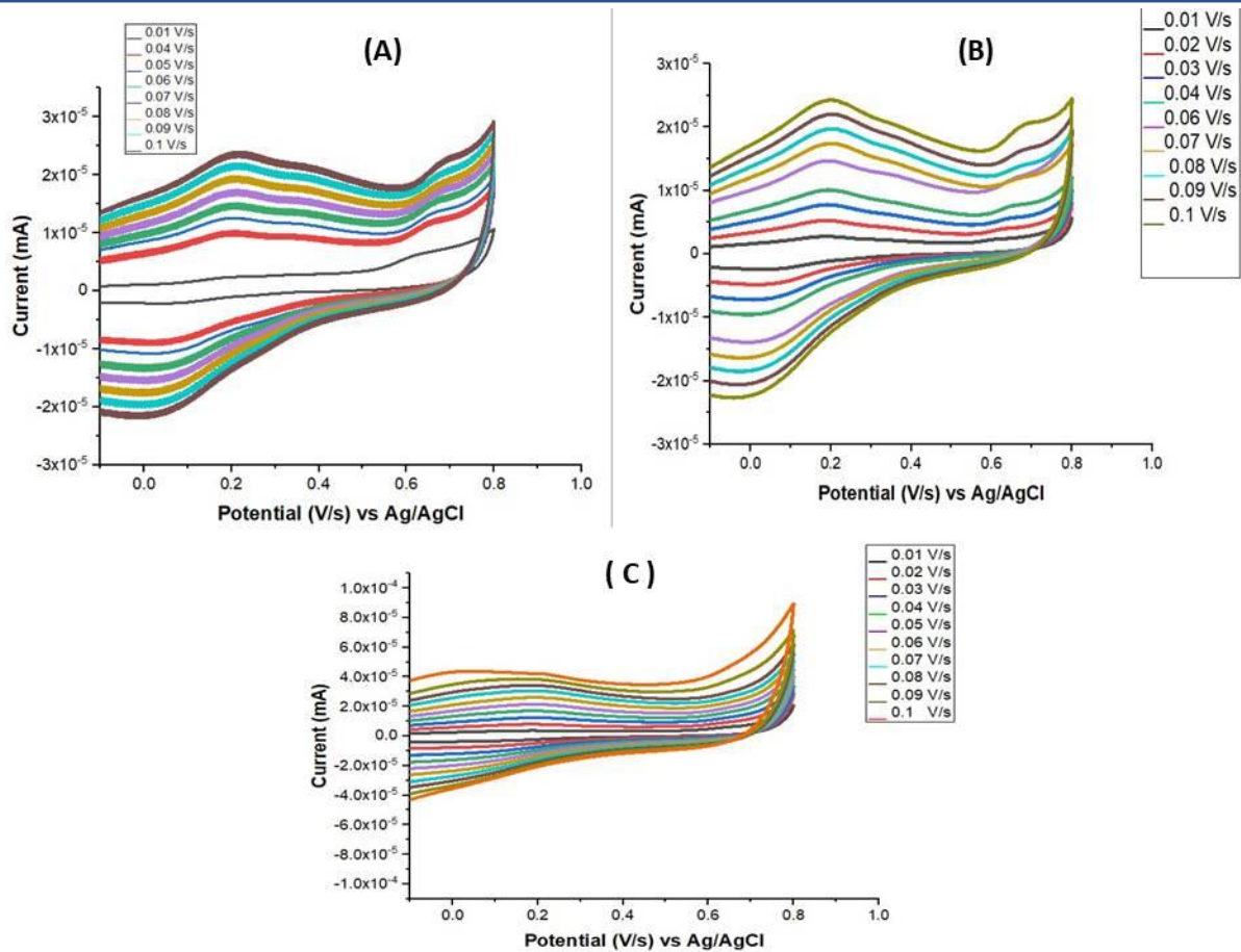
Figure 1. Three different electrodes results against to clavulanic acid and the drug amoxicillin at different scan rates (0.01-0.1 V/s) (A) MWCNT/GCE (B) Fe 3 O 4 @MWCNT NPs/GCE (C) GCE.
