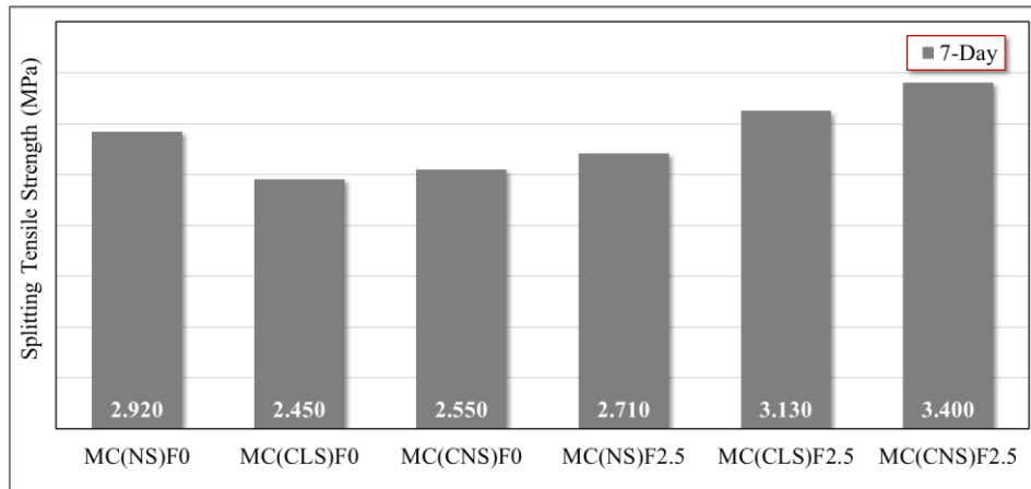
Figure 9. Variation of splitting tensile strength
