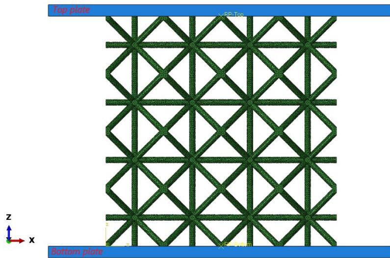
Figure 2. FE model of the BCC unit cell lattice structure
