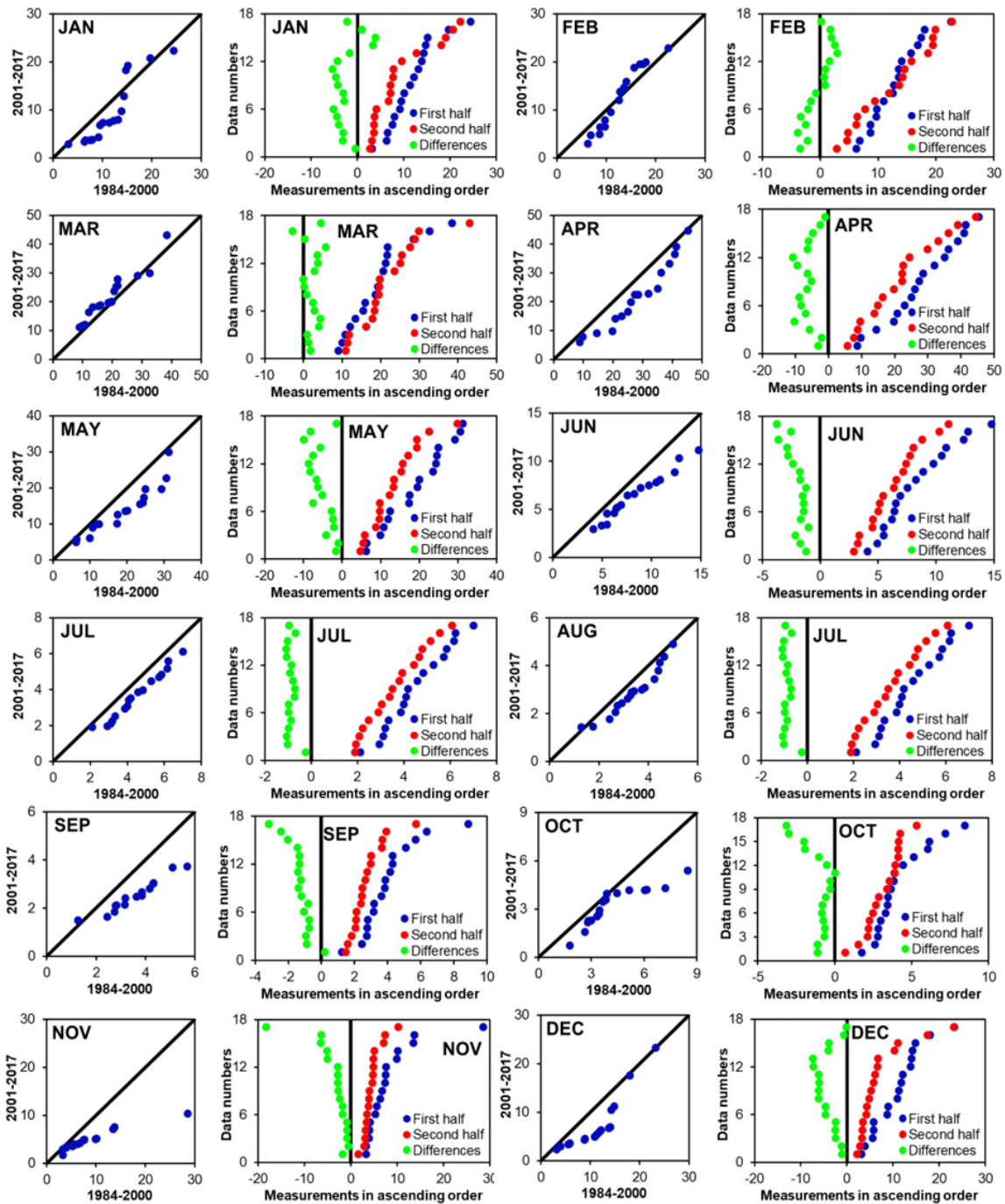
Figure 4.2. Classic Şen-ITA and VATA graph for monthly average flow data
