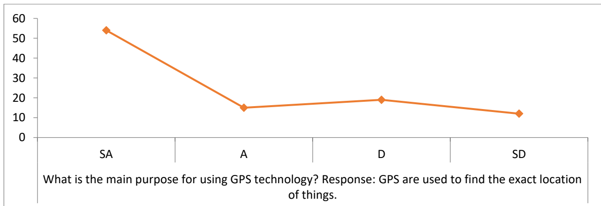
Fig.2: Chat Analysis
