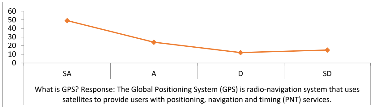
Fig.1: Chat Analysis
