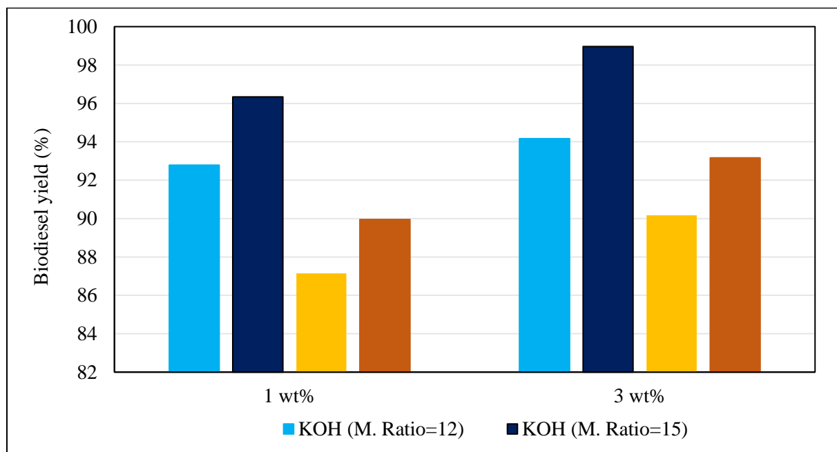
Figure 2. Biodiesel yield values with respect to catalyst amounts, molar ratios and catalyst types
