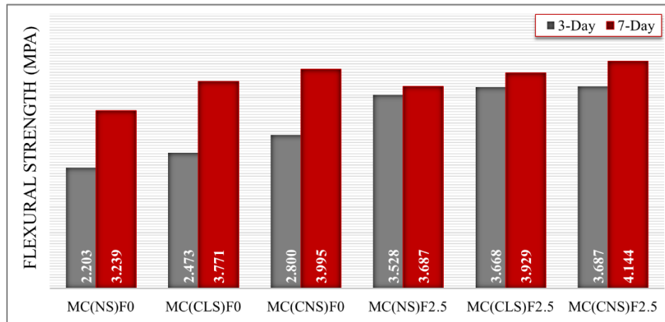
Figure 7. Variation of flexural tensile strength for 3 and 7 days
