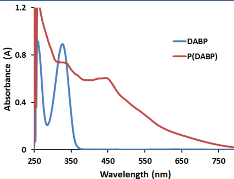
Figure 2. UV-Vis spectra of DABP and P(DABP) (solvent: DMSO)
