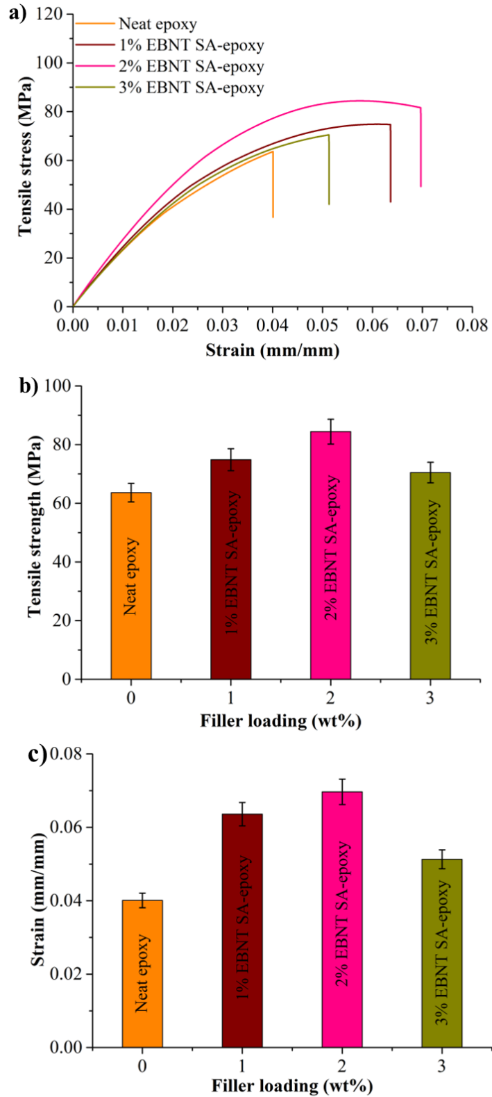
Figure 3.1. a) Tensile stress-strain curves, b) tensile strength, and c) strain values of neat epoxy and EBNT SA-epoxy nanocomposites
