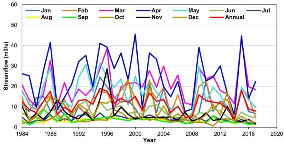
Figure 2.1. Time series of annual and monthly flow data for the period 1984-2017
