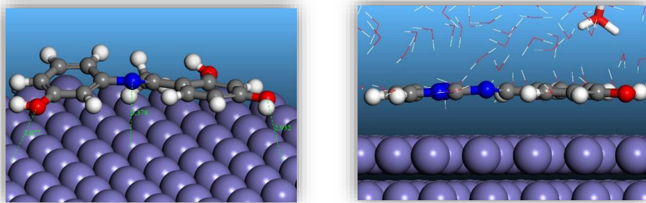
Fig 1: Side views of the most stable adsorption configuration for the Fe (110) / MA9 / 491 H 2 O / (9H 3 O + ,9Cl - ) system obtained by Mont Carlo simulations.
