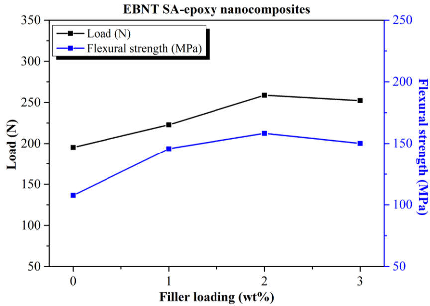
Figure 3.2. Flexural test results of neat epoxy and EBNT SA-epoxy nanocomposites
