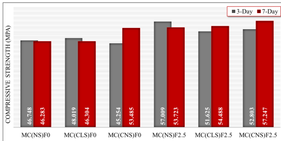
Figure 8. Compressive strength variation at 3 and 7 days
