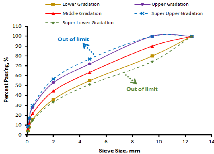
Figure 2.1. Gradation curves of the asphalt mixtures
