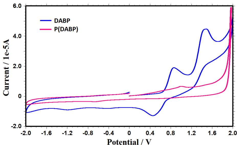
Figure 5. Cyclic voltammograms of DABP and P(DABP)
