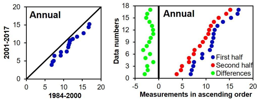
Figure 4.1. a) Classical Şen-ITA, b) VATA graph for annual average flow data
