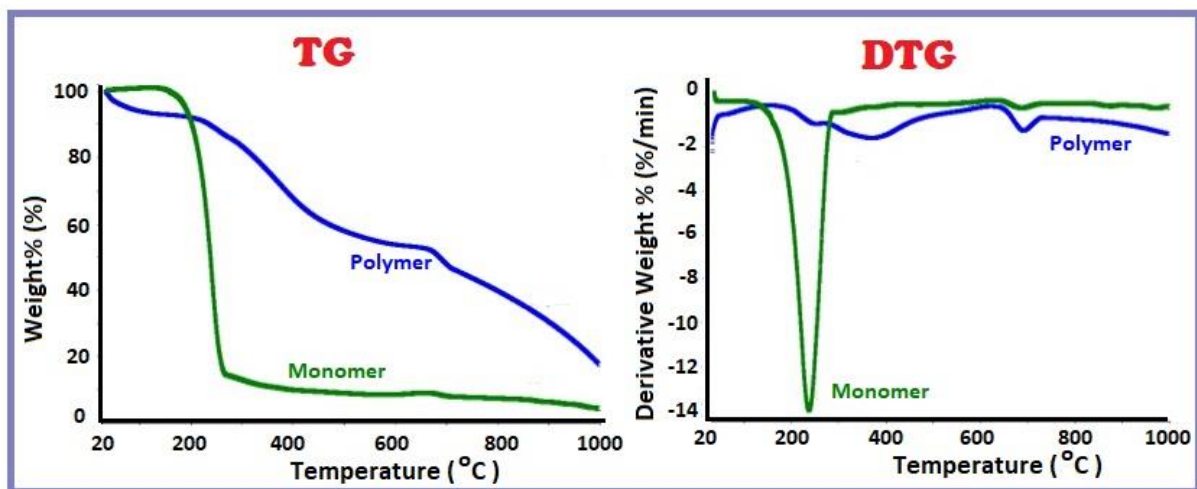
Figure 6. TG and DTG curves of DABP and P(DABP)
