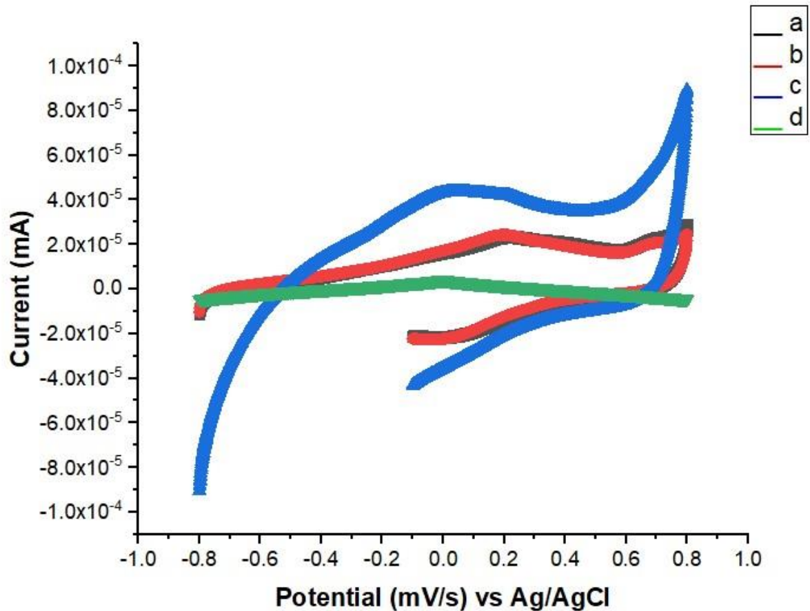
Figure 2. The different electrodes results against to same drug concentration at 0.1 V/s scan rate (a-b) MWCNT/ GCE ( c ) \text{Fe}_3\text{O}_4 @MWCNT/GCE (d) GCE.
