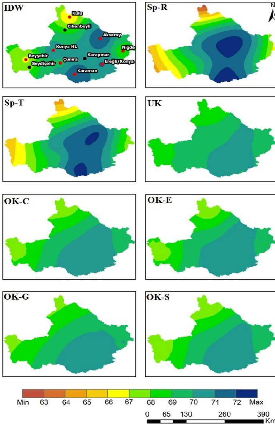
Figure 4.2. Spatial distribution maps of monthly total PET for the period 1971-2019
