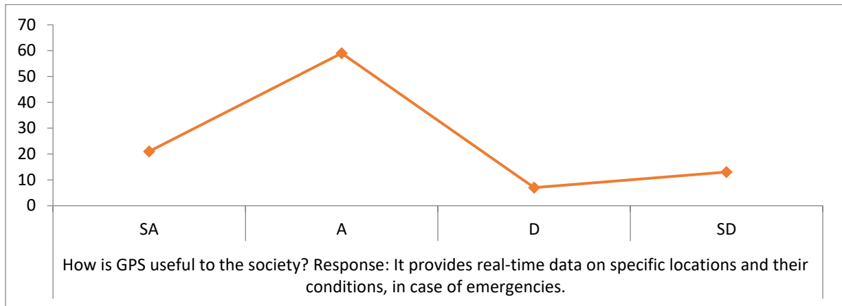
Fig.3: Chat Analysis
