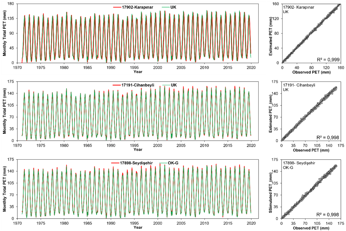
Figure 4.1. Monthly total PET time series and scatter diagrams of observations and model for the period 1971-2019
