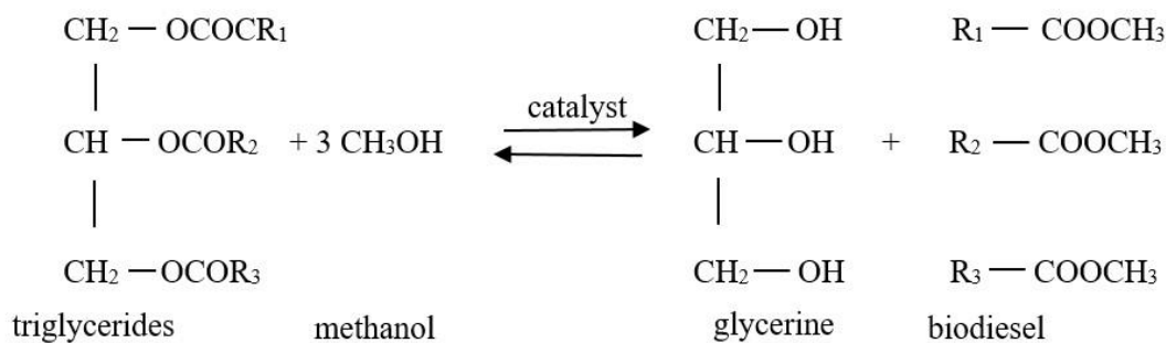
Figure 1. Transesterification reaction
