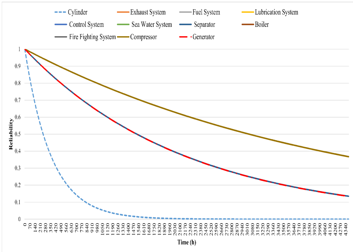
Figure 3. The reliability of each component existed in the engine room
