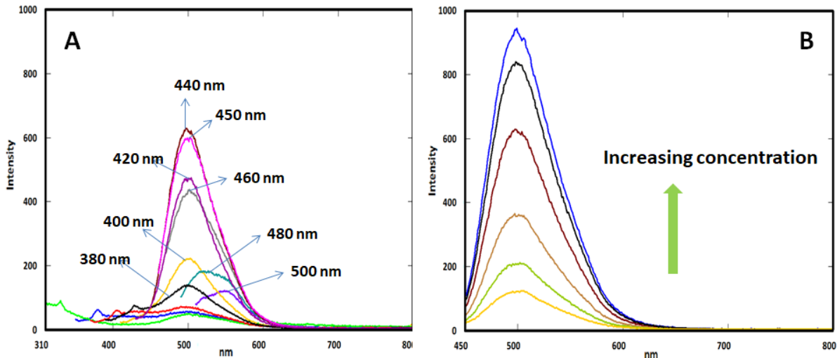
Figure 4. A) P(DABP) emission intensity versus wavelength of excited light B) Dependence of emission intensity on the concentration of P(DABP)
