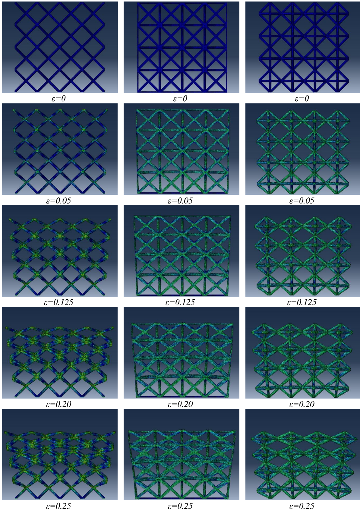
Figure 5 Deformation patterns of base lattice structures
