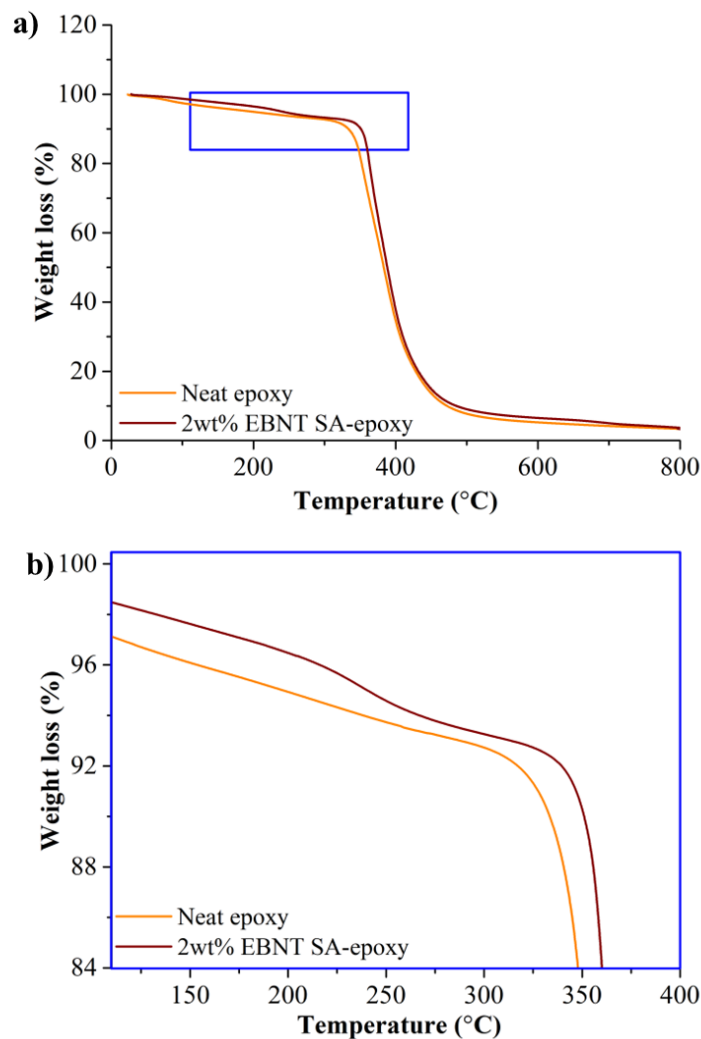
Figure 3.4. TGA curves of neat epoxy and 2wt% EBNT SA-epoxy nanocomposite
