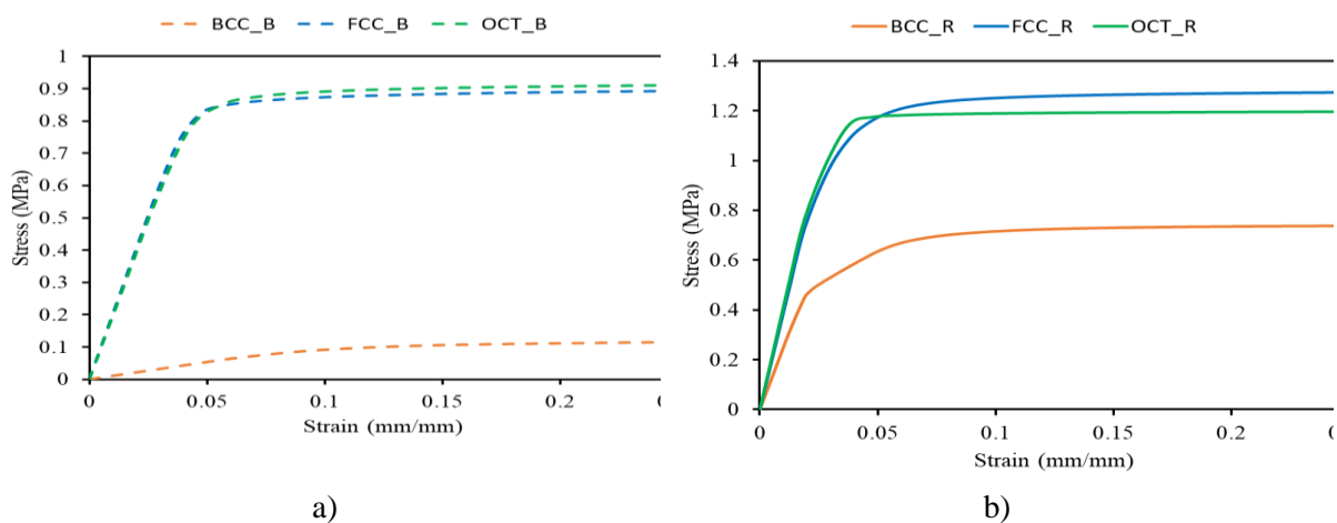
Figure 4 Stress-strain diagrams of a) base b) reinforced lattice structures
