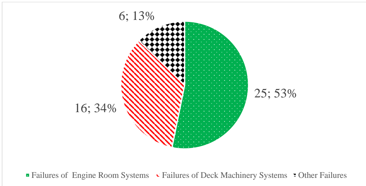
Figure 1. Failures of Ships based on ship systems
