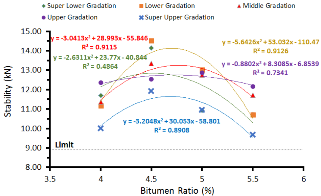
Figure 2.2. Marshall stability results of the mixtures
