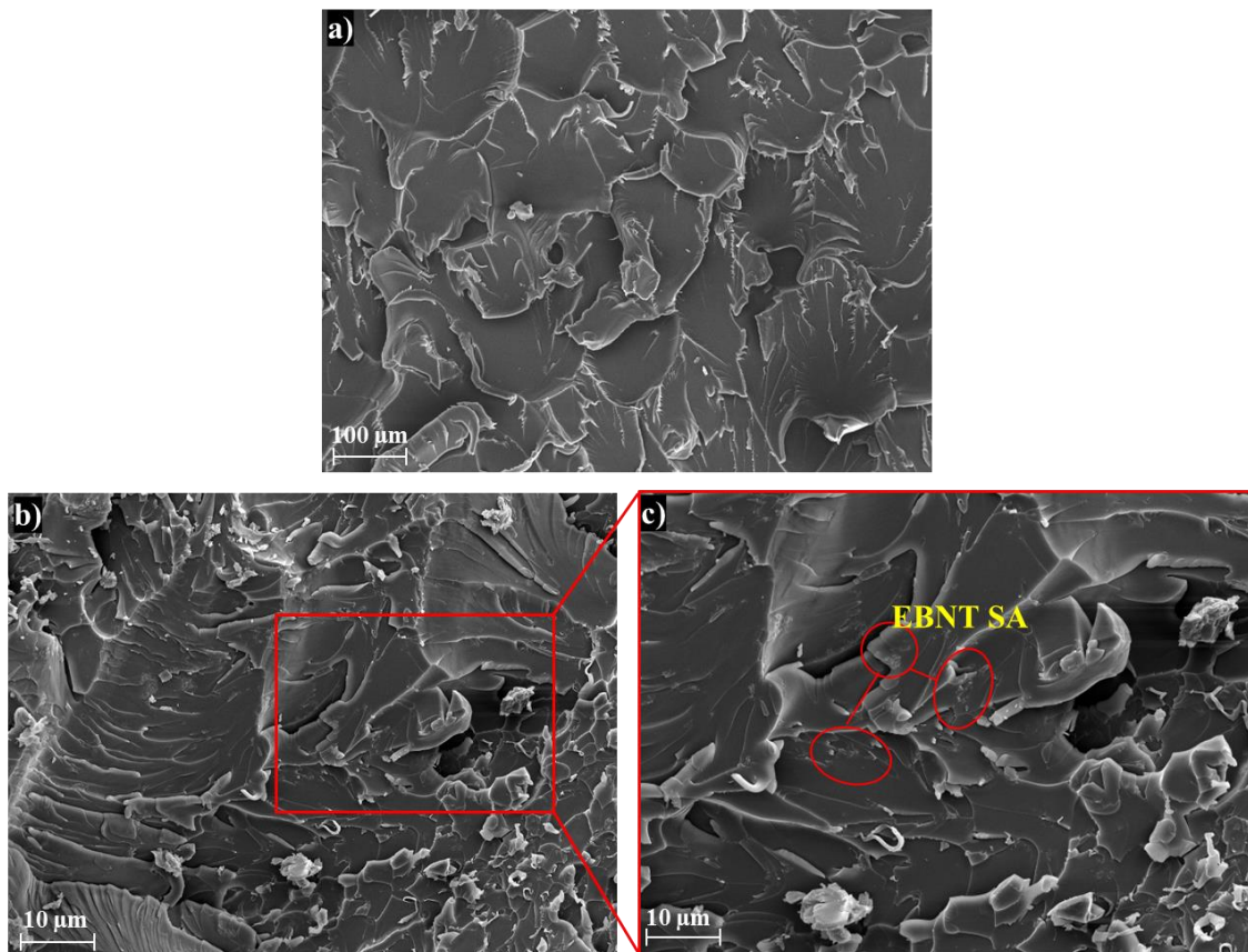
Figure 3.3. SEM images of tensile fractured surfaces of neat epoxy and EBNT SA-epoxy nanocomposites
