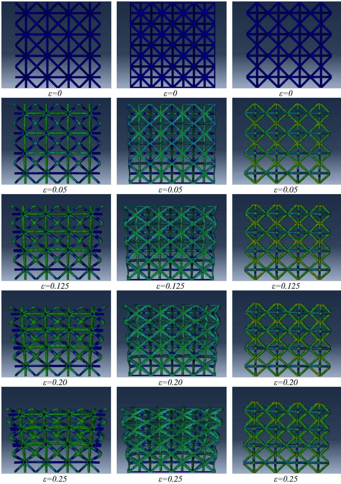
Figure 6 Deformation patterns of reinforced lattice structures
