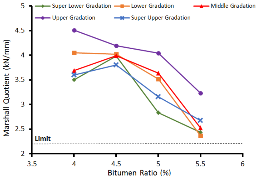
Figure 2.4. Marshall Quotient values of the mixtures
