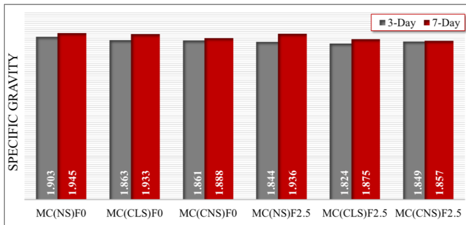
Figure 6. Unit volume weight change for 3 and 7 days
