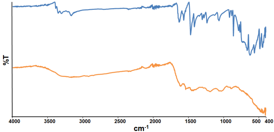
Figure 1. FTIR spectra of DABP and P(DABP)
