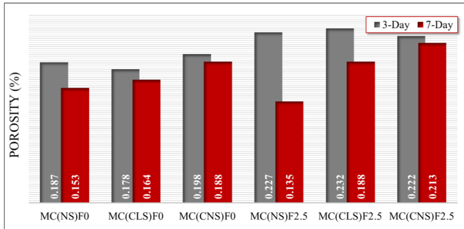
Figure 5. 3- and 7-days porosity change
