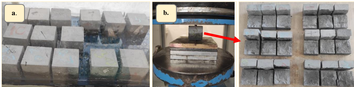
Figure 3. a. capillary water absorption test b. splitting tensile test
