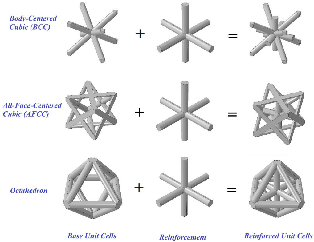
Figure 3. CAD models of strut based unit cells
