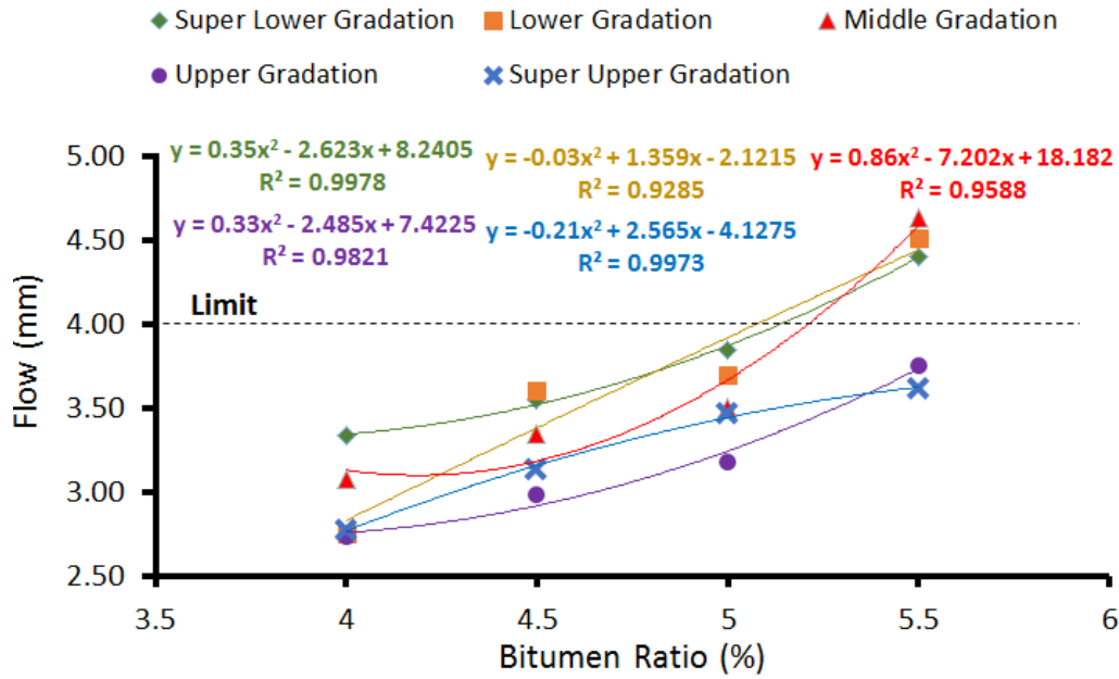
Figure 2.3. Marshall flow results of the mixtures
