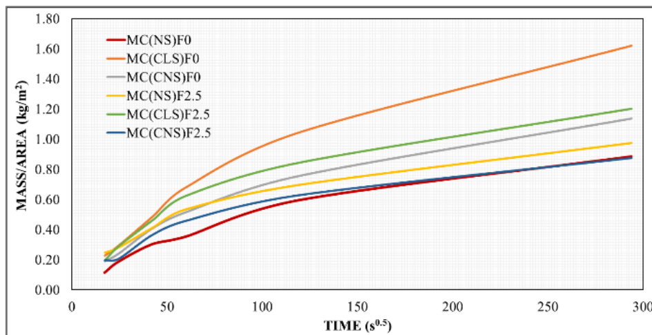
Figure 10. Sorptivity test results
