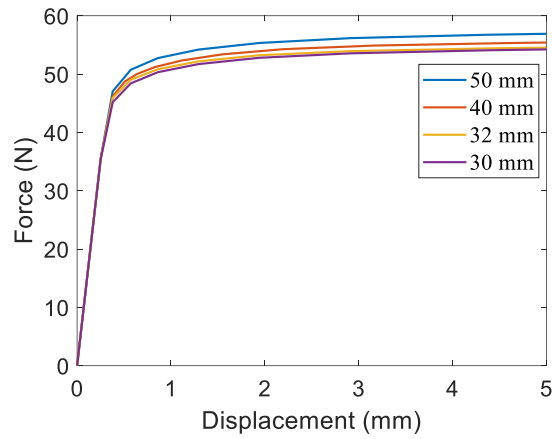
Figure 1 Mesh convergence study of the single BCC unit cell.
